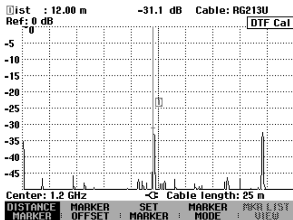
Measurement with automatic setting of the span Measurement with 400 MHz span (span = 2.025 GHz)
